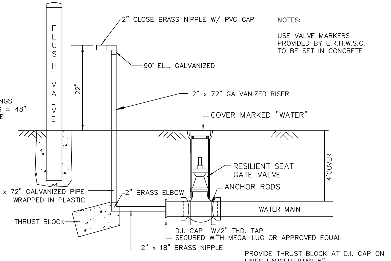
FLUSH VALVE ON FULL SIZE LINE VALVE DETAIL WATER LINE CONSTRUCTION N.T.S.
