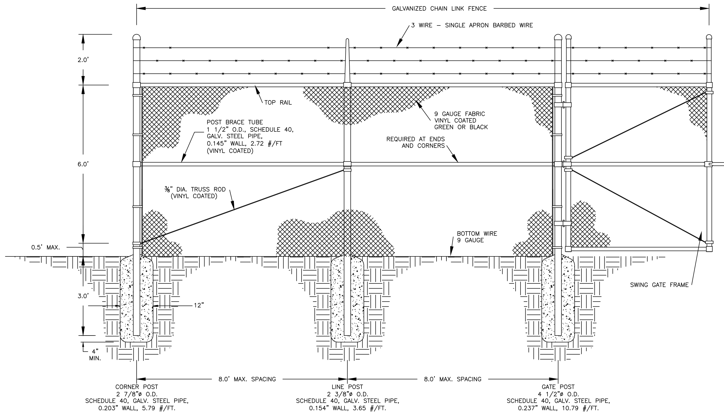
LIFT STATION FENCE DETAIL N.T.S.
