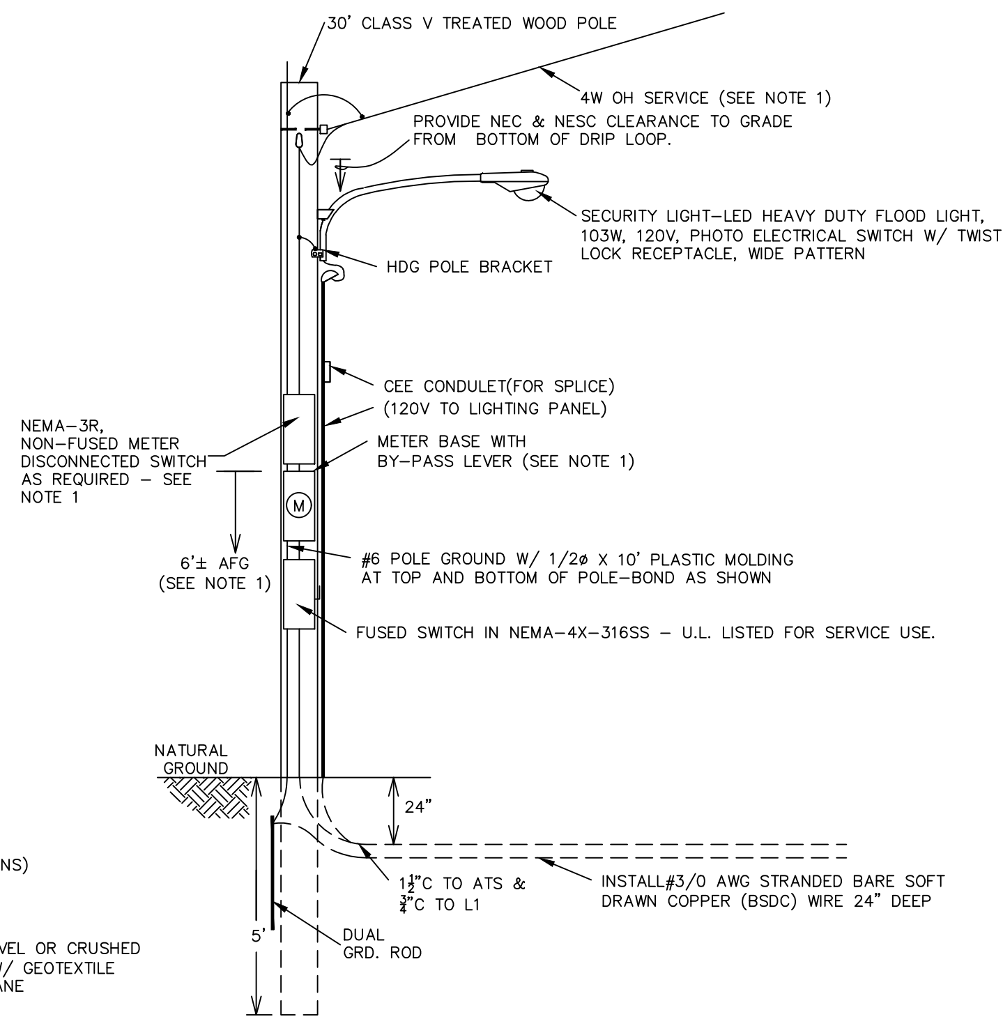
PROPOSED SERVICE POLE DETAIL N.T.S.
