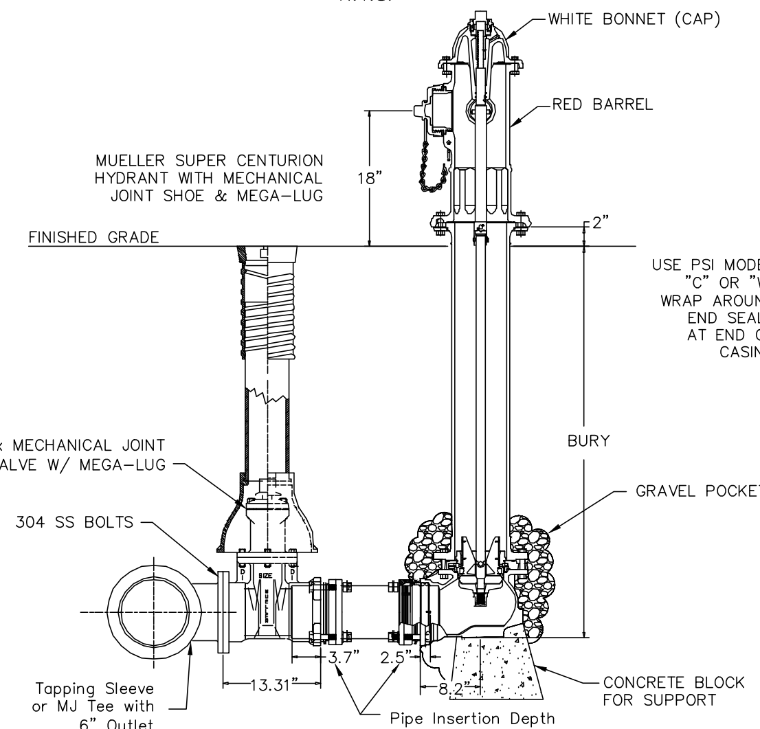
FIRE HYDRANT ASSEMBLY N.T.S.
