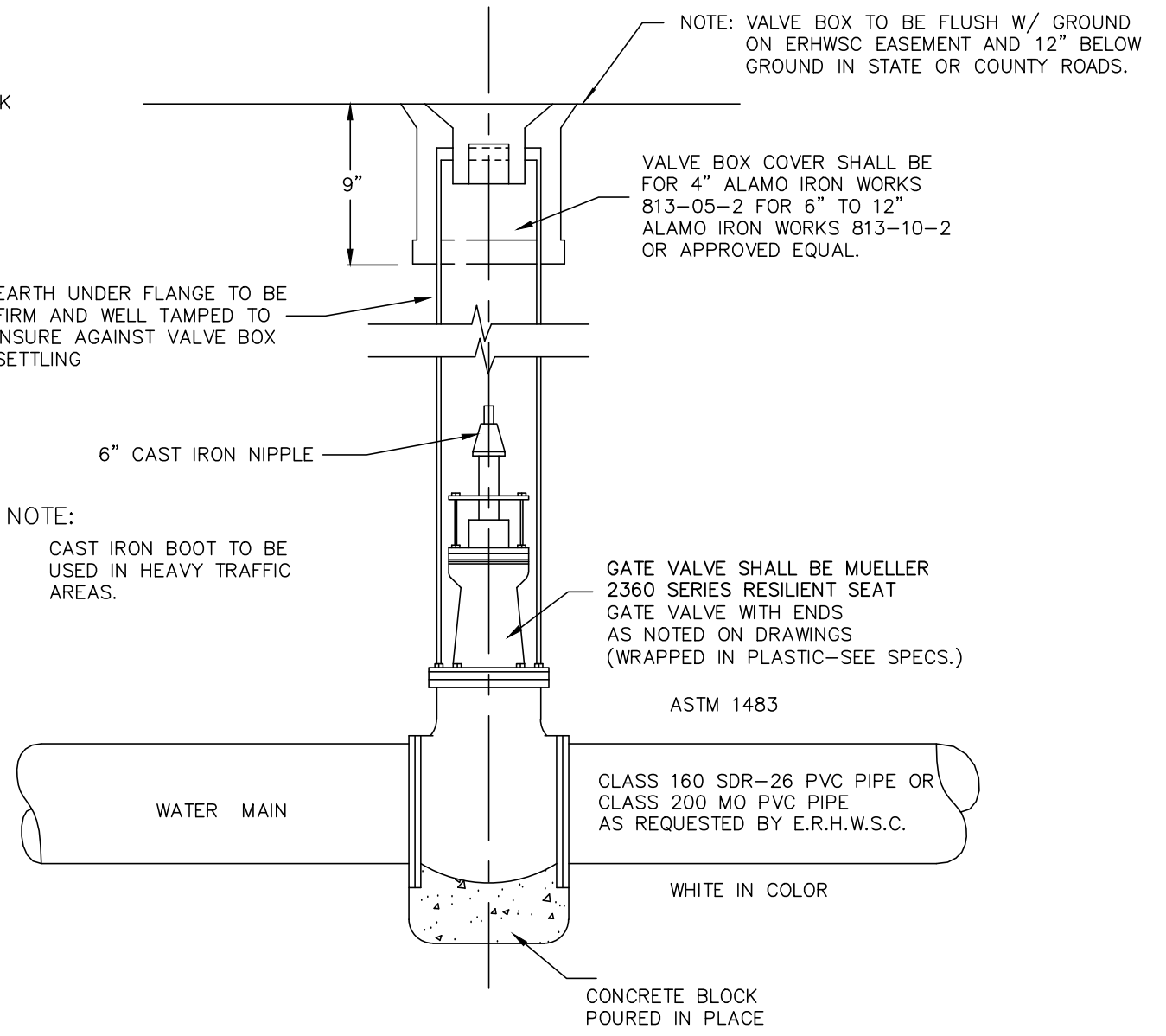
TYPICAL VALVE AND VALVE BOX INSTALLATION ON MAIN LINE N.T.S.
