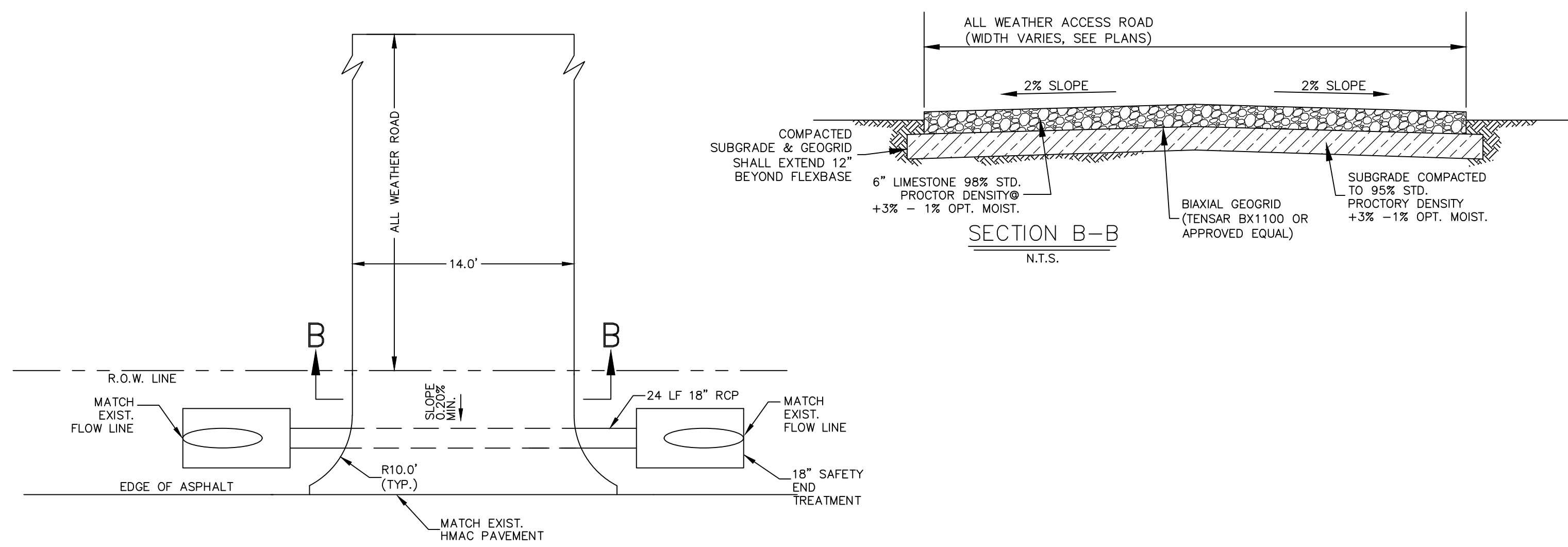
TYPICAL LIFT STATION DRIVEWAY APRON N.T.S.
