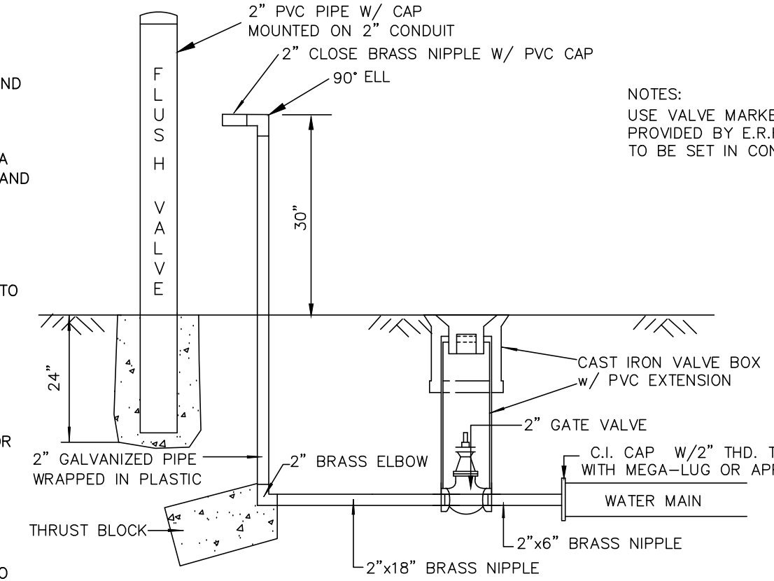
FLUSH VALVE DETAIL W/2" VALVE WATER LINE CONSTRUCTION N.T.S.
