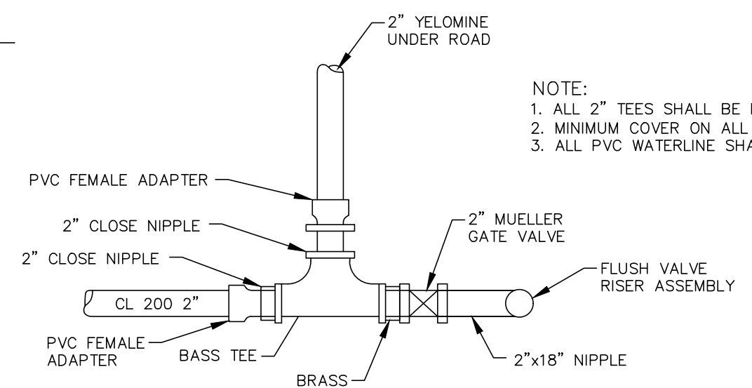
FLUSH VALVE DETAIL ON 2" LINE IN CUL DE SAC N.T.S.
