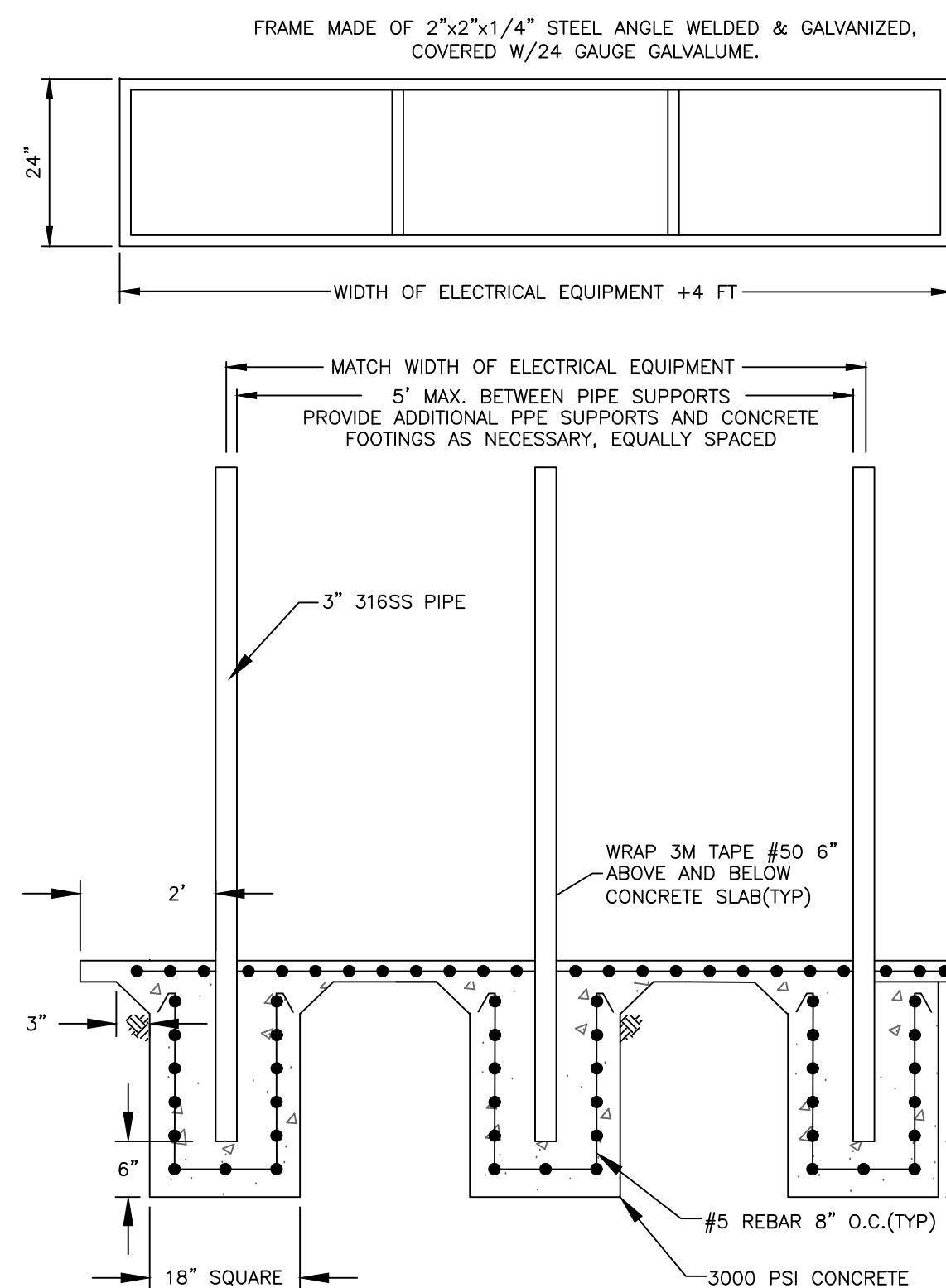
TYPICAL RACK SUPPORT & ROOFING DETAIL NOT TO SCALE
